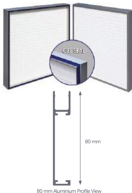
80 mm Aluminium Profile View
