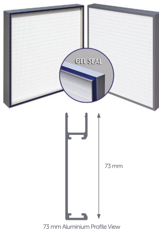
73 mm Aluminium Profile View
