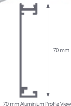
70 mm Aluminium Profile View
