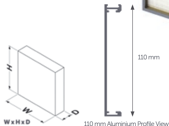
110 mm Aluminium Profile View
