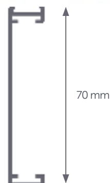
70 mm Aluminium Profile View
