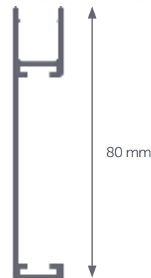
80 mm Aluminium Profile View
